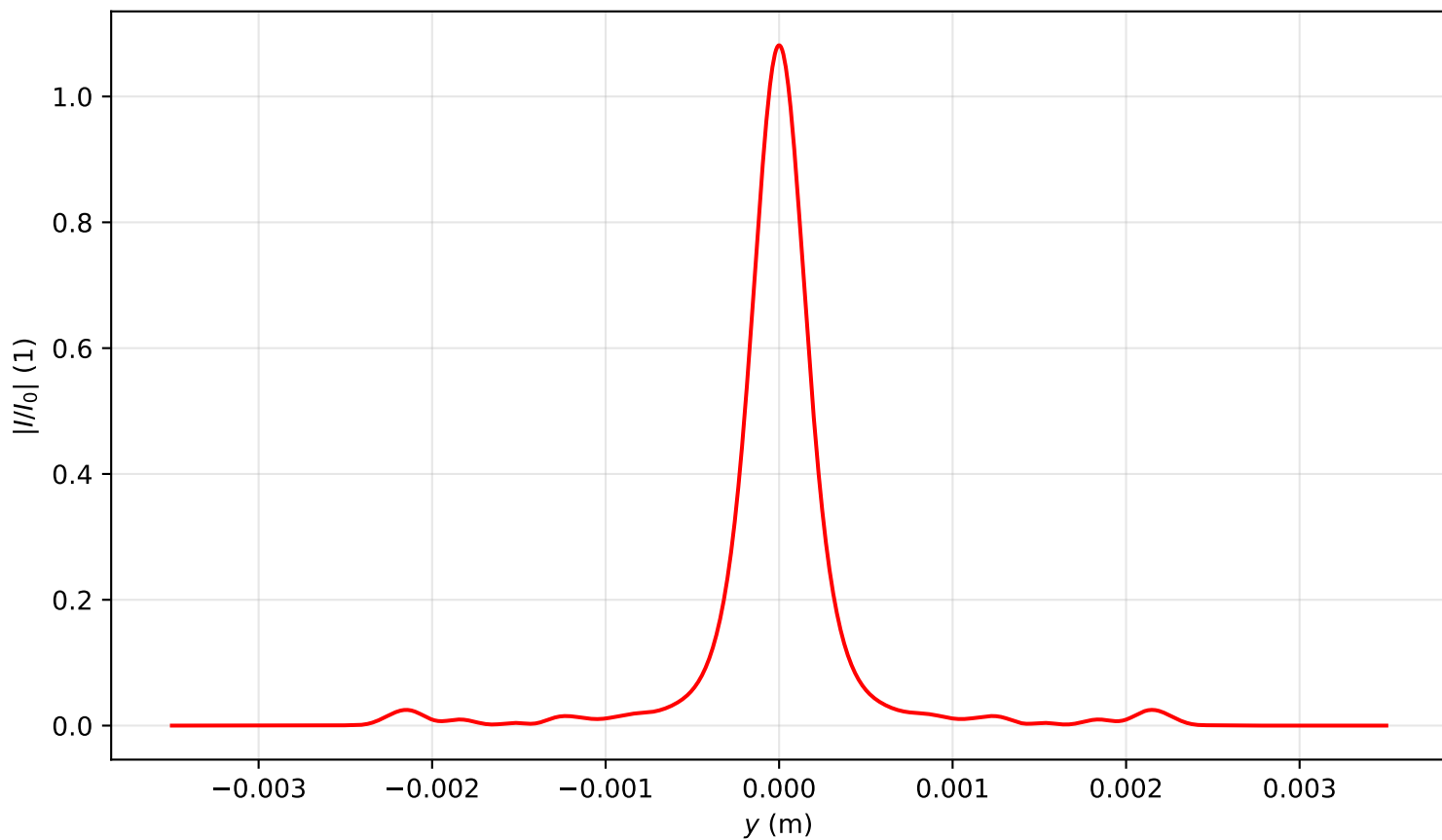
Intensity profile I(x=0, y, z=3.821)/I_0 , P_{in}=3.5P_{cr} , artificial time
